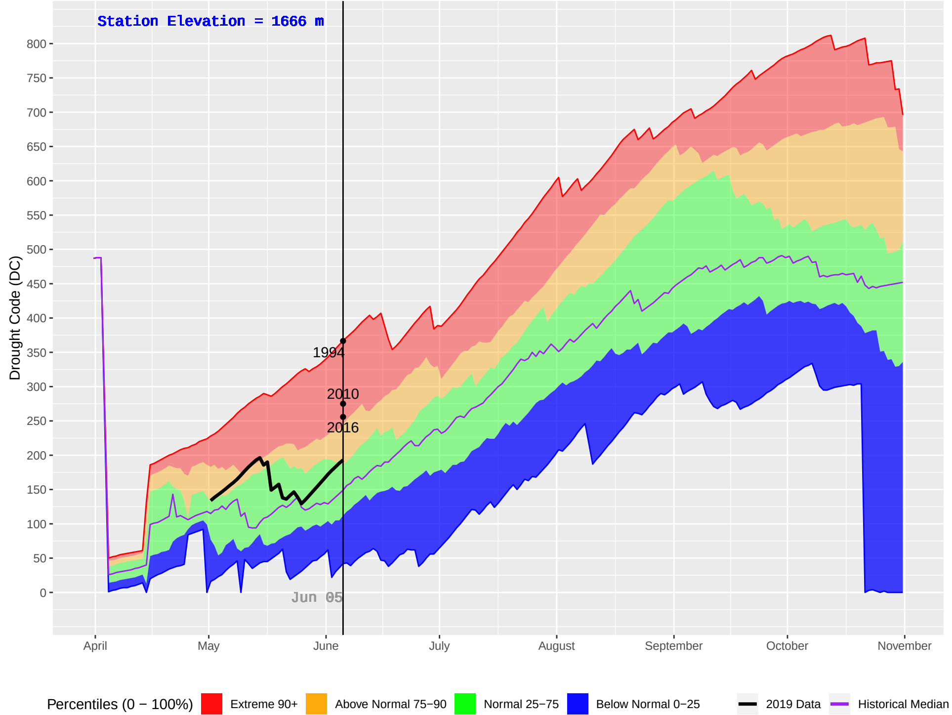
BALDFACE (221) : Historical (1992–2018) and Current (2019) Daily Drought Code (DC)
