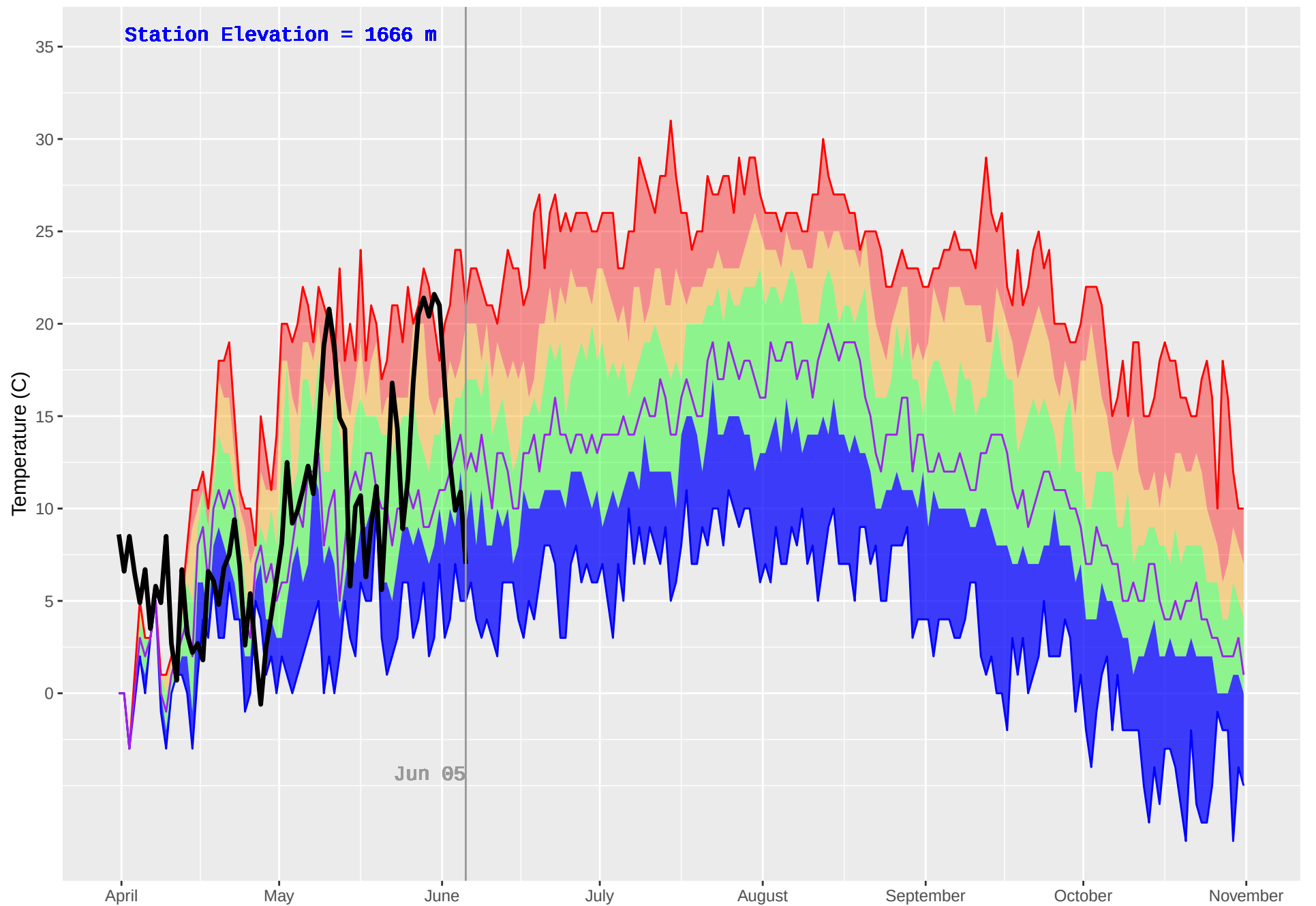
BALDFACE (221) : Historical (1992–2018) and Current (2019) Daily Temperature
