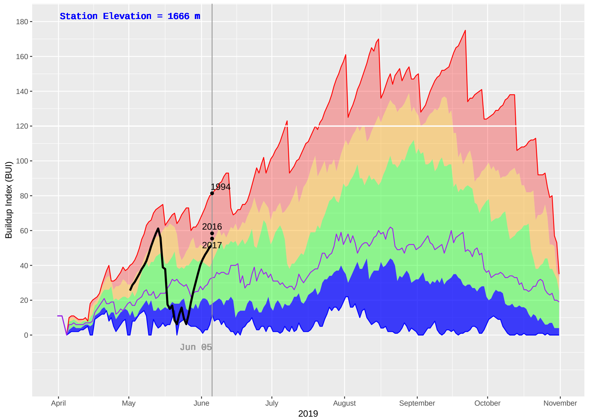
BALDFACE (221) : Historical (1992–2018), Current (2019) Daily Buildup Index (BUI)
