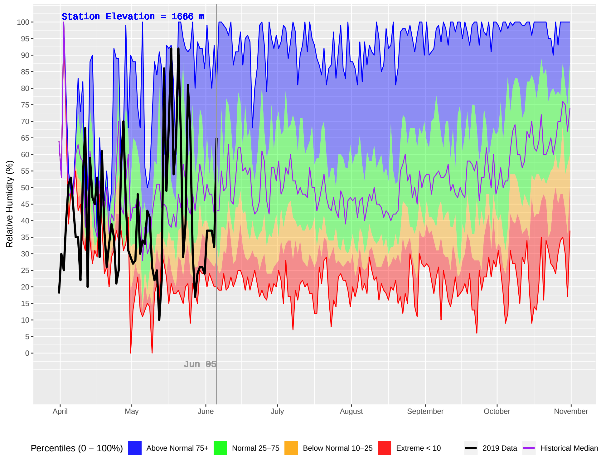
BALDFACE (221) : Historical (1992–2018) and Current (2019) Daily Relative Humidity
