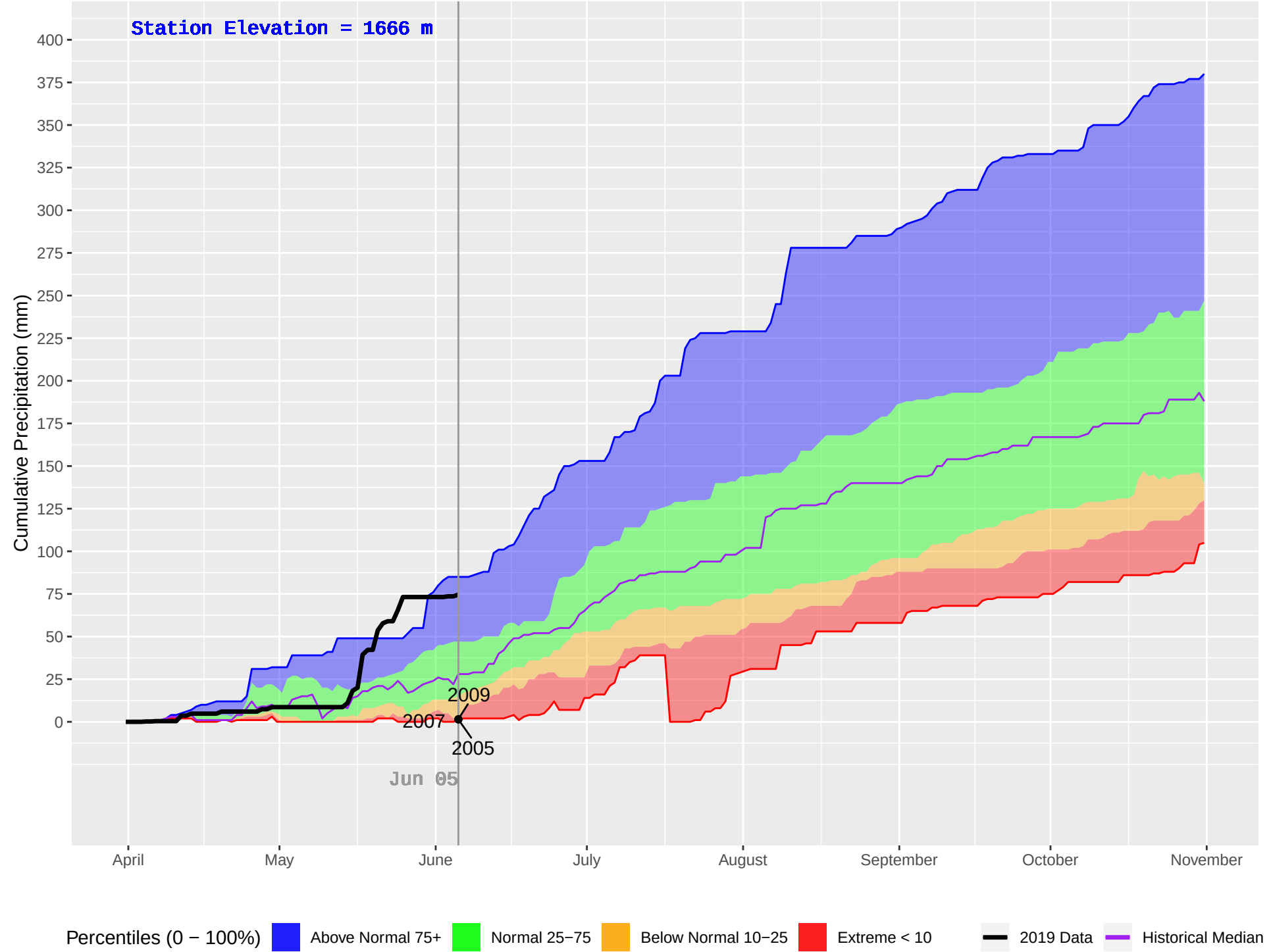
BALDFACE (221) : Historical (1992–2018), Current (2019) Daily Cumulative Precipitation
