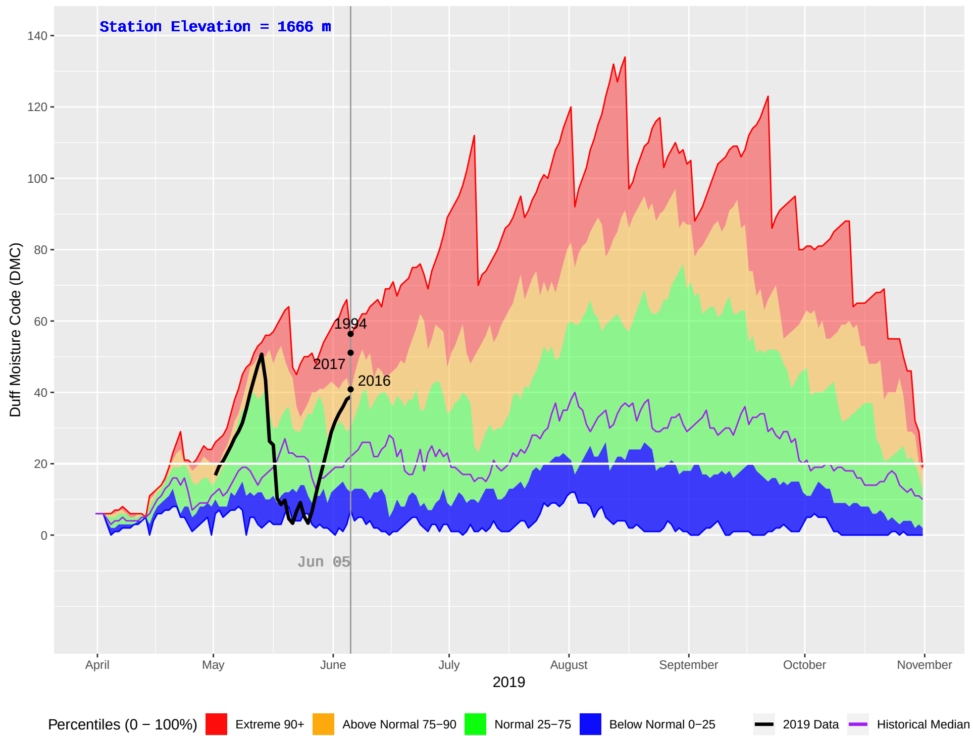
BALDFACE (221) : Historical (1992–2018), Current (2019) Daily Duff Moisture Code (DMC)
