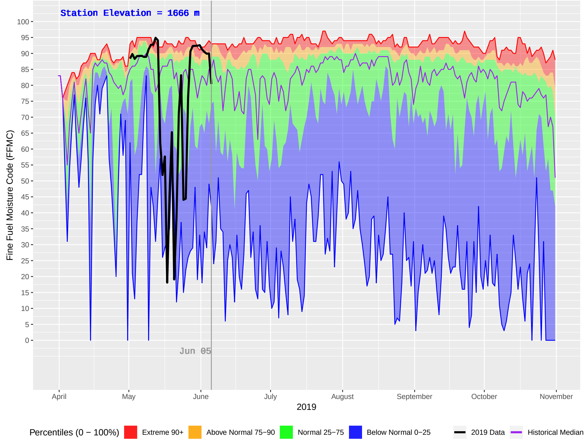
BALDFACE (221) : Historical (1992–2018) and Current (2019) Daily Fine Fuel Moisture Code (FFMC)
